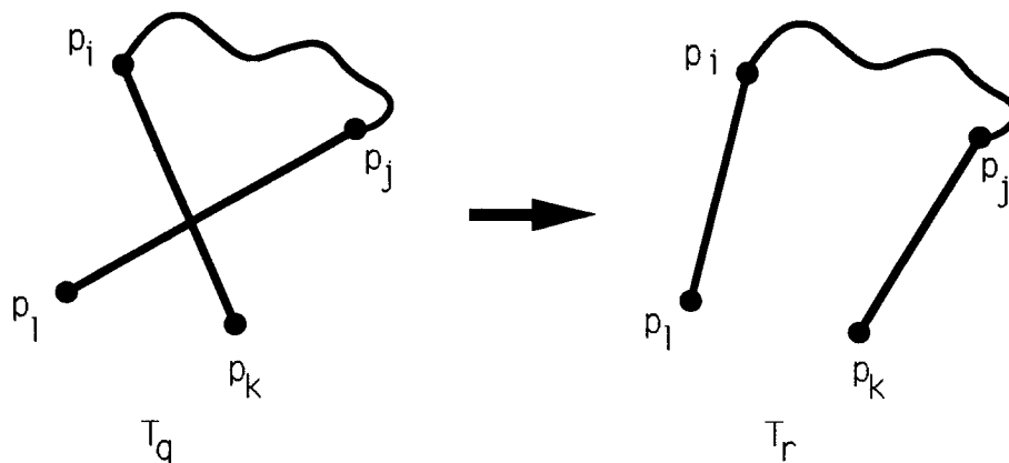
Figure 2.1: Example if crossed lines are in a single 1-tree
