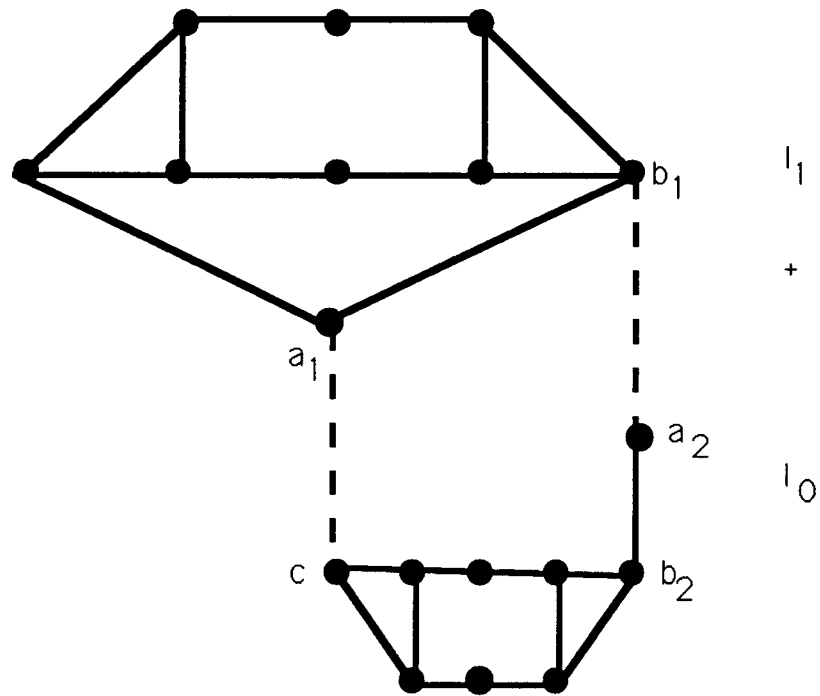
Figure 4.2: Instance I_2 = I_1 + I_0
