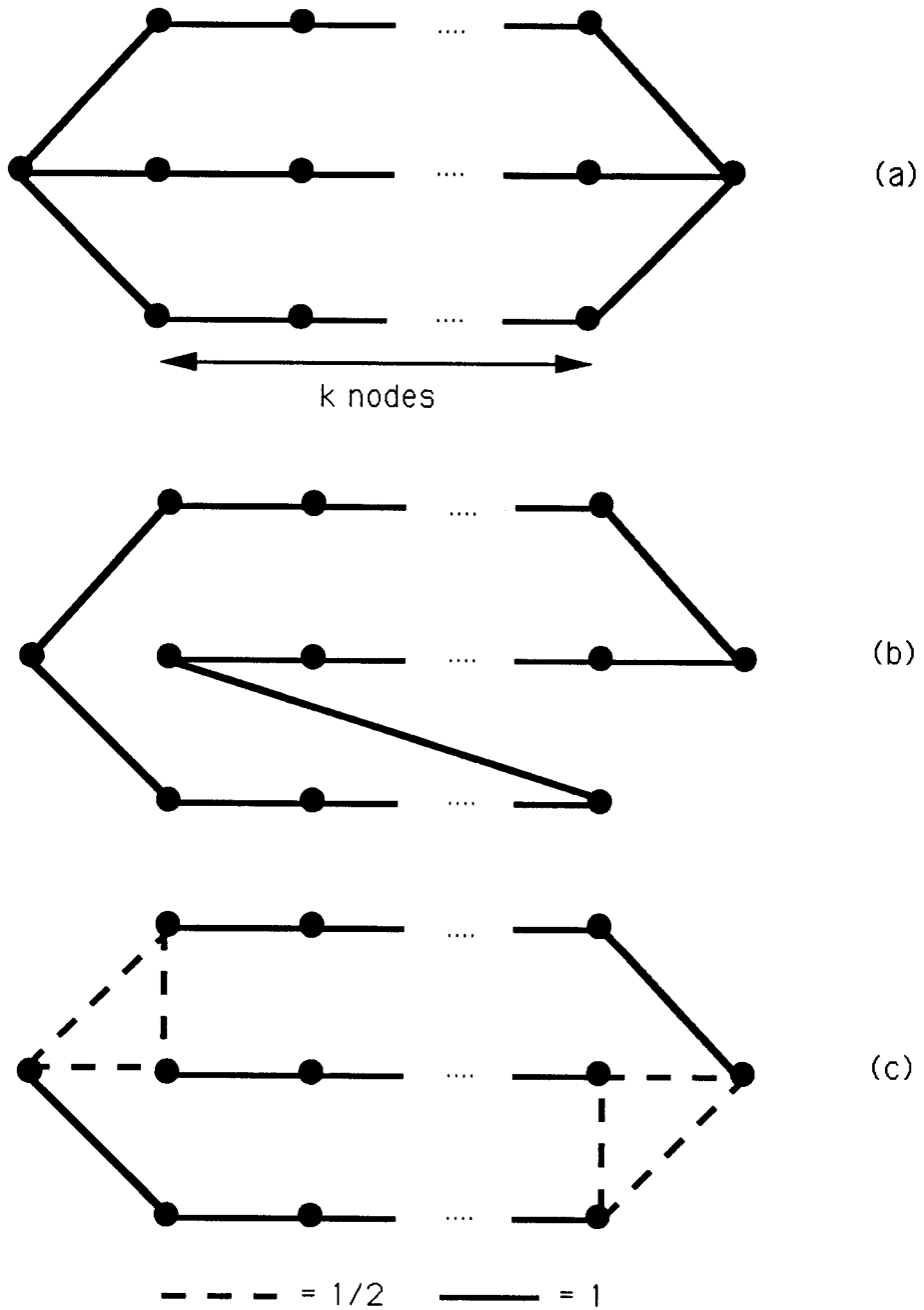
Figure 2.3: Conjectured Worst Case for the Held-Karp Heuristic
